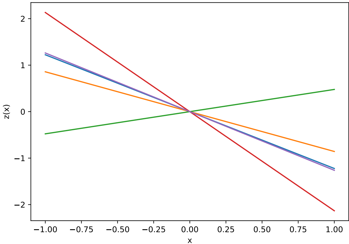
GP - Linear kernel
